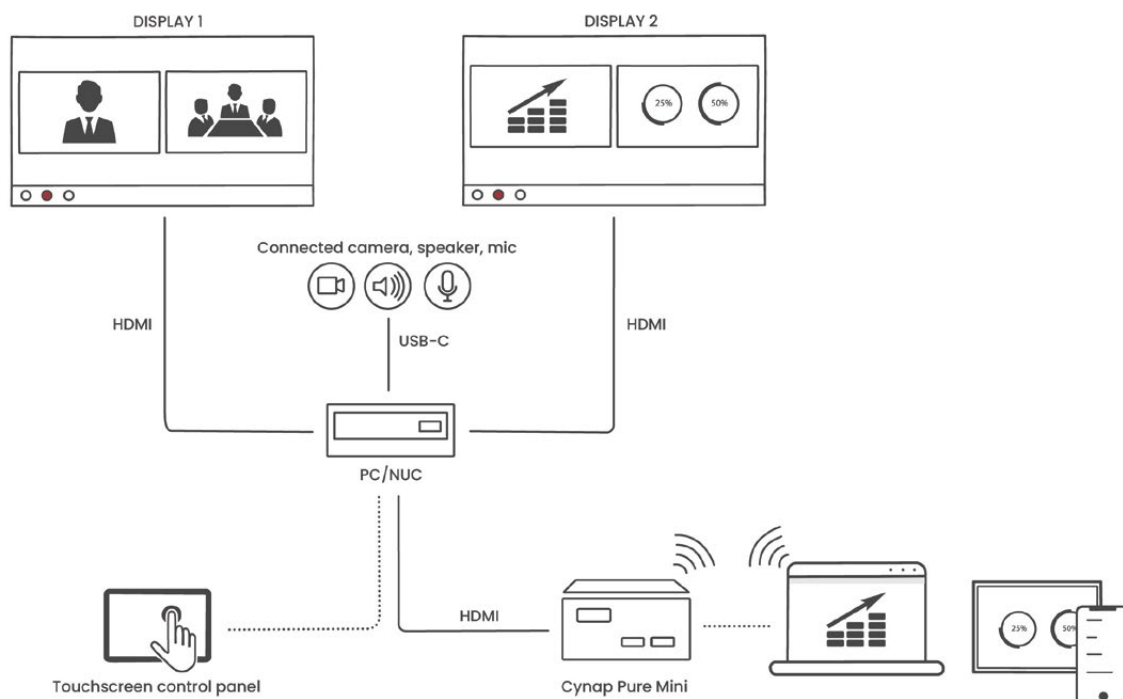
Sample setup: Cynap Pure Mini used as a plug-in to a Zoom /Teams room to provide high-performance wireless screen sharing.
